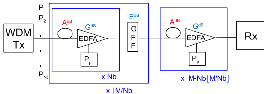
Figure 5. Block diagram of a sparse-GFF link, obtained by concatenating no-GFF blocks of size N_b , with GFFs in between them, up to a total M span link. All fiber spans have the same loss A . All EDFAs in the link have the same physical parameters and pump.
