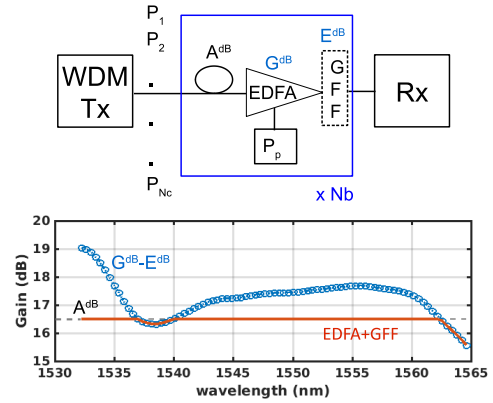
Figure 1. (Top) Single-mode WDM short link with N_c = 40 channels and N_b spans, span attenuation A and co-pumped single-stage EDFAs with optical pump power P_p . In the un-flattened case, no GFF is present. In the gain-flattened case, every EDFA is followed by a GFF with excess loss E > 1 . (Bottom) Sketch of the EDFA unfiltered Gain G at channel locations (circles), decreased by the GFF excess loss, and amplifier gain after the GFF (solid line). The dashed horizontal line indicates the span loss A .
