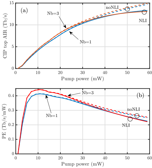
Figure 8. (a) top-AIR for our 40 WDM CIP channels vs. EDFA pump power P_p at optimal EDFA length 5.3m, both for reference all-GFF system ( N_b = 1 ) and for sparse-GFF at optimal block size N_b = 3 . Dashed: no NLI, solid: NLI. 287 spans, span loss A = 9.5 dB, span length 50.9km, PSCF fiber. (b) Power efficiency PE = \text{top-AIR}/P_p versus P_p . GFF loss 0.3dB.
