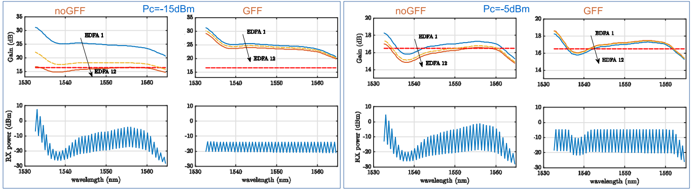
Figure 3. (top row) Gain at EDFAs 1, 12 (solid) and block-average gain (dashed) and (bottom row) RX power vs. wavelength, for a single block of N_b = 12 spans, span loss A = 16.5\text{dB} , doped fiber length \ell = 8.3\text{m} , 40 WDM channels (bandwidth 50GHz, spacing 100GHz), at pump powers P_p = 25\text{mW} . Both the GFF (zero excess loss) and the no-GFF cases are shown, at both a small TX power ( P_c = -15\text{dBm} ) and the GFF-top-AIR power ( P_c = -5\text{dBm} ).
