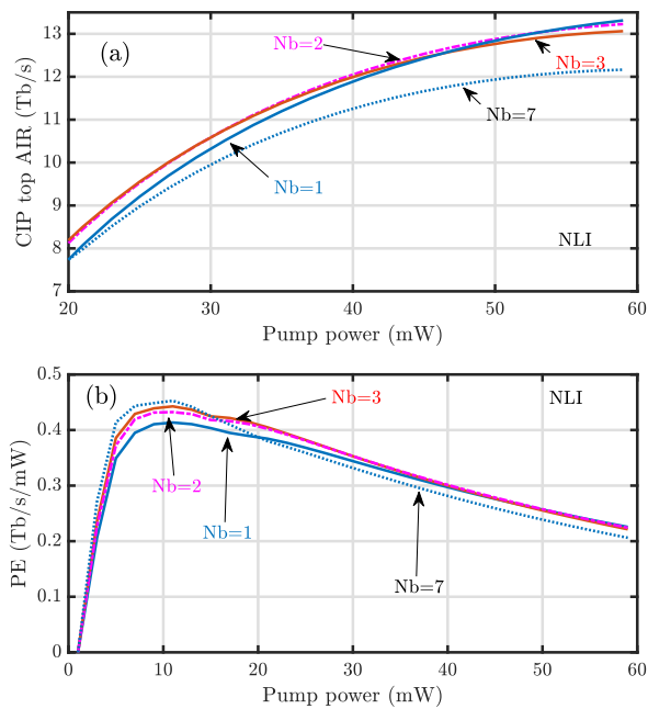
Figure 10. Same as Fig. 8 (only NLI case) but we added the N_b = [2, 7] cases. GFF excess loss 0.3dB.
