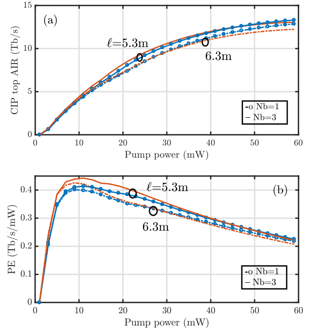
Figure 9. (a) top-AIR for our 40 WDM CIP channels vs. EDFA pump power P_p at both optimal EDFA length 5.3m (solid) and sub-optimal length 6.3m (dash-dot), both for all-GFF reference system ( N_b = 1 , circles) and sparse-GFF optimal block size N_b = 3 . M=287 spans, span loss A = 9.5 dB, span length 50.9km, including NLI from PSCF propagation. (b) corresponding power efficiency PE = \text{top-AIR}/P_p versus pump power.
