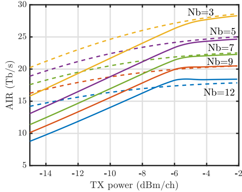
Figure 4. AIR (Tb/s) vs. P_c (dBm) for blocks of length [3, 5, 7, 9, 12] spans, 40 WDM CIP channels, pump P_p = 25\text{mW} , span loss A = 16.5\text{dB} , EDFA length \ell = 8.3\text{m} . no NLI. Solid: GFF with excess loss 0.3dB; dashed: no-GFF.
