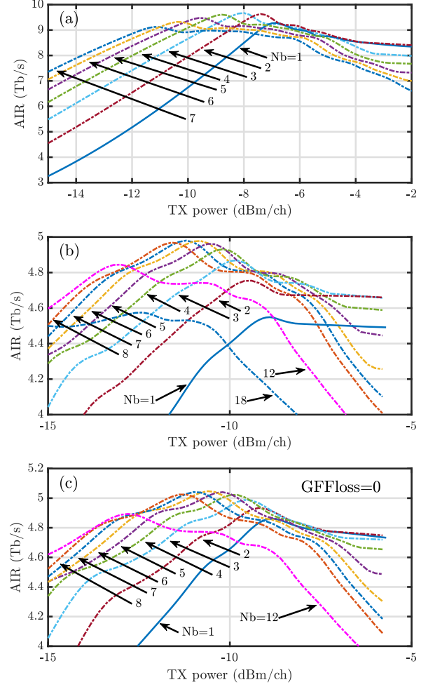
Figure 7. AIR vs. P_c for transmission of 40 WDM CIP channels over 287 spans, span loss A = 9.5 dB, EDFA length \ell = 5.3 m, at various sparse-GFF block sizes N_b ( N_b = 1 is the reference all-GFF link). (a) P_p = 25 mW, GFF loss 0.3 dB (b) P_p = 11 mW, GFF loss 0.3 dB; (c) P_p = 11 mW, zero GFF loss. NLI included.
