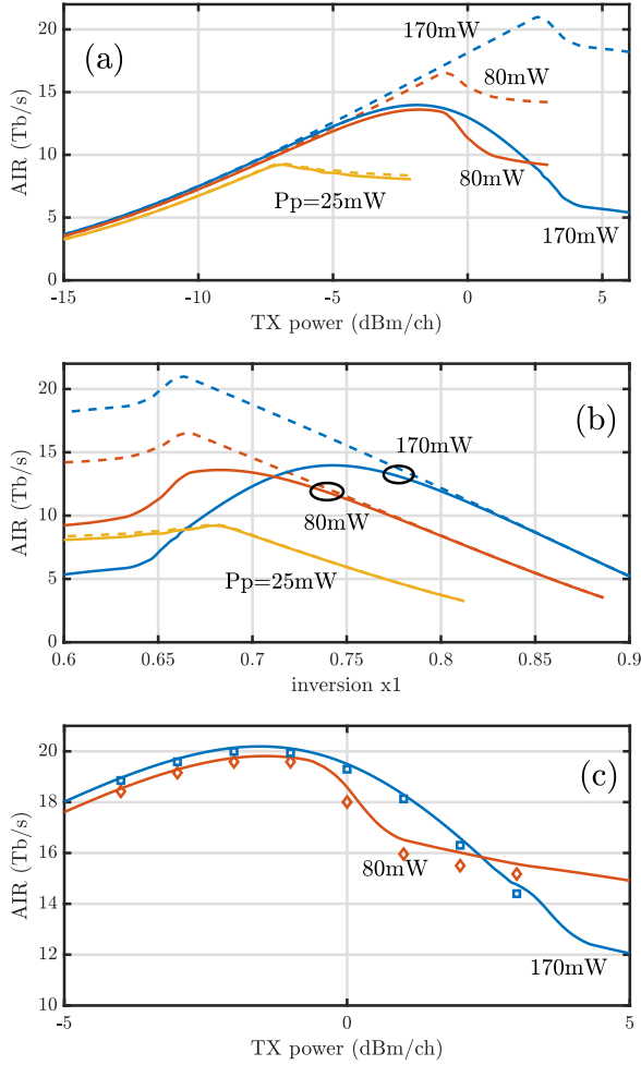
Figure 6. (a) AIR vs. P_c and (b) AIR vs. inversion x_1 of the first EDFA, for a reference GFF link ( N_b = 1 ) with 287 spans, span loss A = 9.5 dB, span length 50.9 km, EDFA length \ell = 5.3 m, 40 WDM channels, at pump powers P_p = [25, 80, 170] mW. Dashed: no NLI; Solid: with NLI on a PSCF fiber; span loss margin 1.25 dB. GFF excess loss 0.3 dB. (c) AIR vs. P_c at 100 spans and same data as above, at P_p = [80, 170] mW, with NLI. Solid: theory. Circles: split-step simulations.
