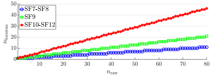
Fig. 15: Number of CoRE Link Format-encoded LoRaWAN packets as a function of the number of raw packets to be sent, for various values of the SF.
