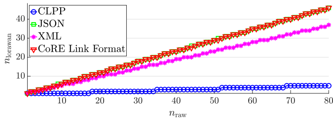
Fig. 18: Number of LoRaWAN packets as a function of the number of raw packets to be sent adopting a LoRaWAN SF equal to SF10-SF12 (sharing the same maximum payload length \ell_{SF10} = \ell_{SF11} = \ell_{SF12} = 51 bytes), shown for each considered data representation format.
