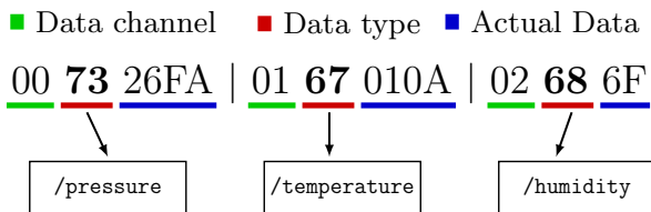
Fig. 2: Example of received CLPP-encoded uplink packet, with corresponding CoAP resources (as detailed in Section 4).
