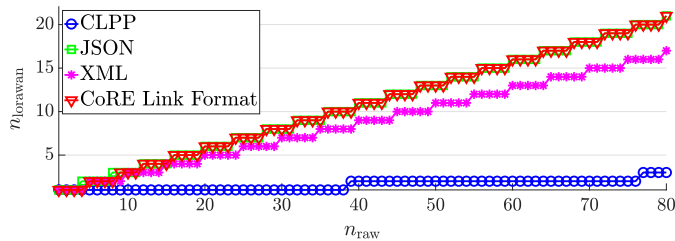
Fig. 17: Number of LoRaWAN packets as a function of the number of raw packets to be sent adopting a LoRaWAN SF9 (having a maximum payload length \ell_{SF9} = 115 bytes), shown for each considered data representation format.
