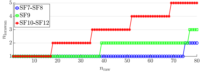
Fig. 12: Number of CLPP-encoded LoRaWAN packets as a function of the number of raw packets to be sent, for various values of the SF.
