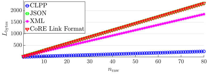
Fig. 11: Number of required bytes as a function of the number of raw packets to be sent, for the chosen data formatting mechanisms: CLPP, JSON, XML, CoRE Link Format.
