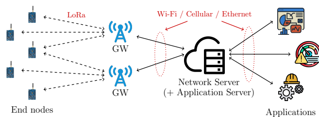
Fig. 1: General LoRaWAN architecture providing IoT-oriented information to external applications.
