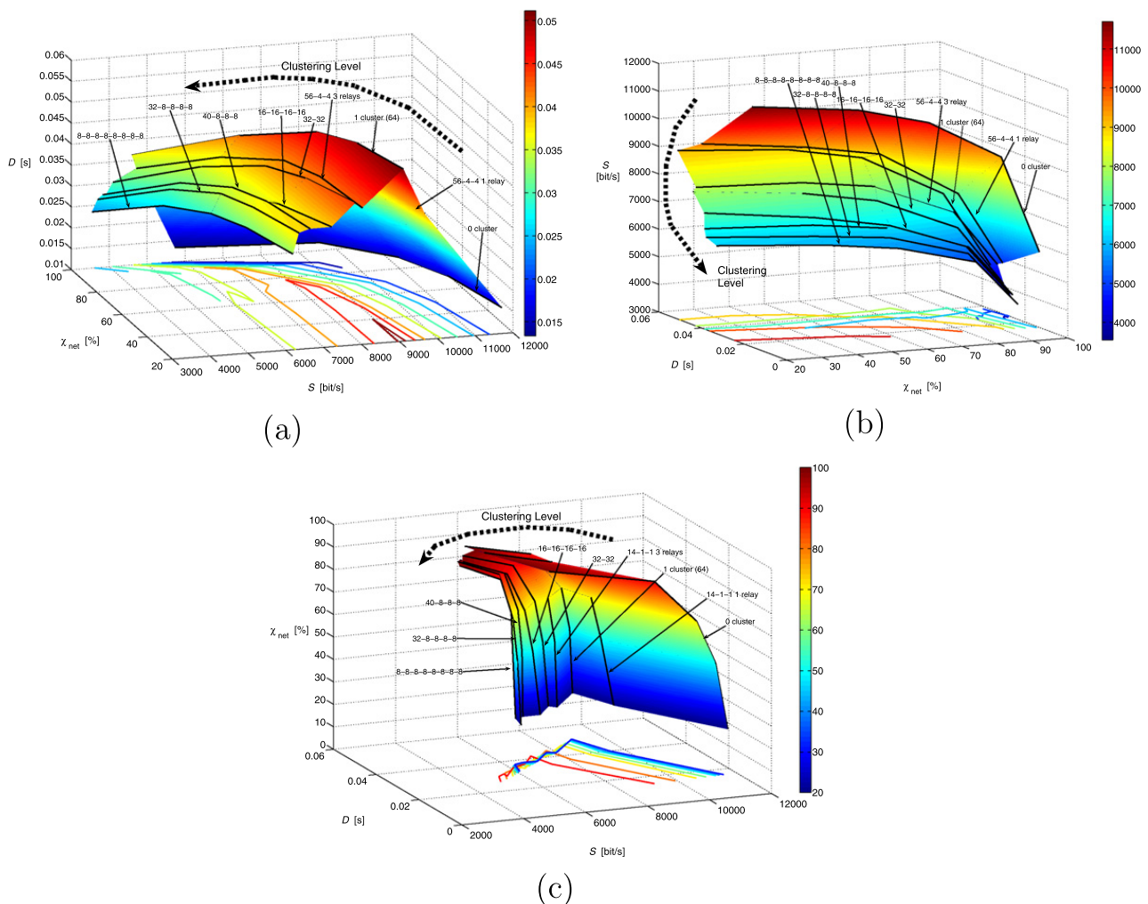
Fig. 17. Performance evaluation in a scenario with N = 64 RFDs and various uniform and non-uniform clustering configurations: (a) delay as a function of network transmission rate and \chi_{net} , (b) network transmission rate as a function of delay and \chi_{net} , and (c) \chi_{net} as a function of network transmission rate and delay. The considered packet generation rate is g = 2 pck/s.
