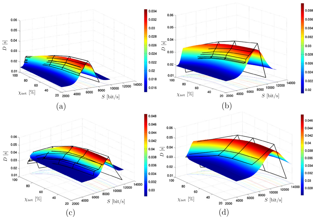
Fig. 18. Performance evaluation in a scenario with the following values of N : (a) 16, (b) 32, (c) 64, and (d) 128. Both the realistic surface (lines) and its approximation (continuous) are shown.
