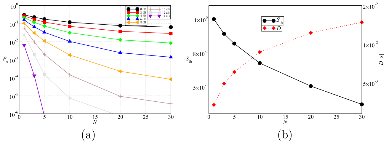
Fig. 13. Performance analysis in a scenario without clustering: (a) probability of decision error at the AP as a function of the number N of transmitting RFDs, considering various SNR at the nodes, and (b) throughput and delay as functions of the number N of transmitting RFDs.
