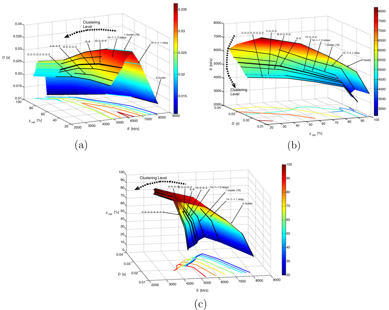
Fig. 16. Performance evaluation in a scenario with N = 16 RFDs and various uniform and non-uniform clustering configurations; (a) delay as a function of network transmission rate and \chi_{net} , (b) network transmission rate as a function of delay and \chi_{net} , and (c) \chi_{net} as a function of network transmission rate and delay. The considered packet generation rate is g = 2 pck/s.
