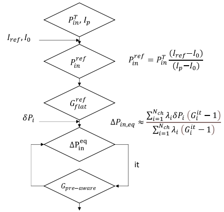
Fig. 1: Extended method to predict G_{pre\ aware}(x)
