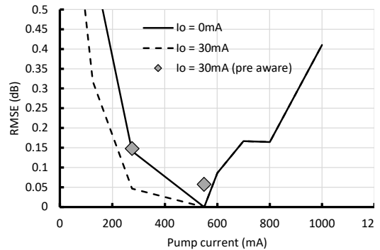
Fig. 5: Experimental RMSE versus EDFA pump current I_p for I_{ref} = 550 mA
