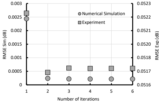
Fig. 4: Graph with RMSE evolution as a function of the number of iterations of the pre-emphasis aware model.
