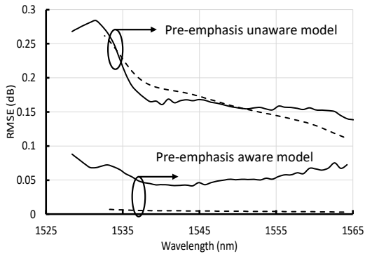
Fig. 2: RMSE versus wavelength: solid lines for experiment and dashed for simulation.
