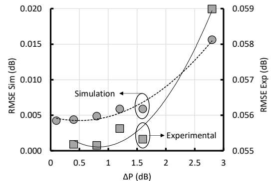
Fig. 3: Evolution of RMSE as a function of \Delta P
