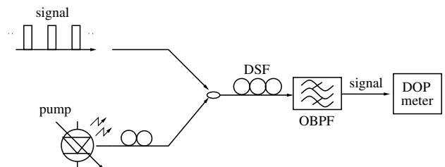
Fig. 1. System setup of a copropagating NLP.
